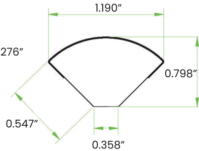
QUARTER ROUND
