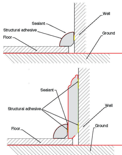
QUARTER ROUND
