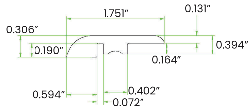
REDUCER
