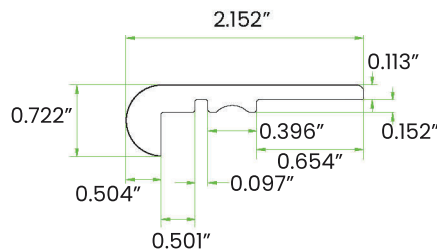
OVERLAP STAIR NOSE
